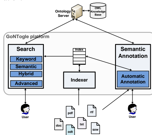
Figure 3. GoNTogle architecture
